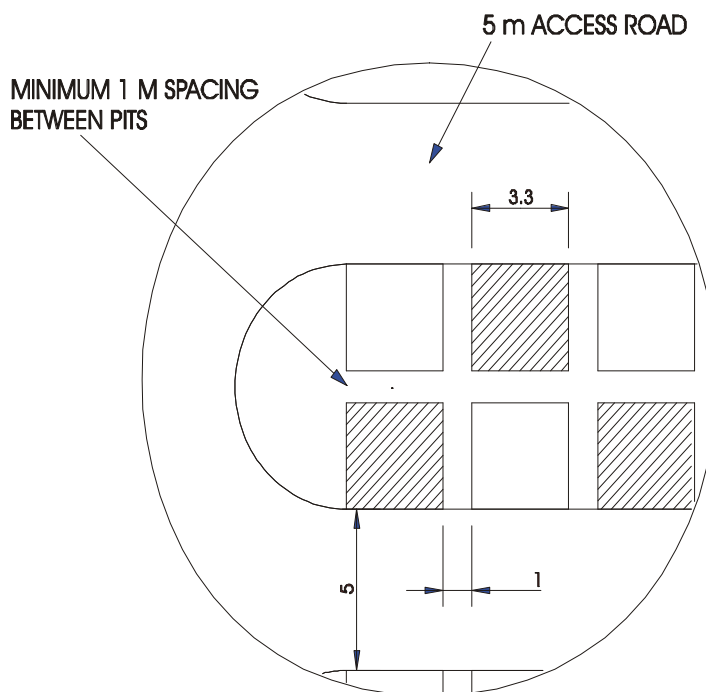
Figure 3: A concept layout pattern for a dedicated faecal waste disposal site
