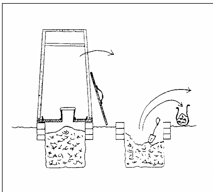
Figure 2: Schematic (from Morgan, 1999) of the Alternating Pit or Fossa Alterna. The pits are sized to fill in 3 to 6 months. When the pit is nearly full, the second pit's contents are emptied and put into compost bags. The latrine structure is moved, and the first pit is topped up with soil and covered. The process can be repeated indefinitely.
